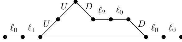
Figure 5: The labeled Motzkin path corresponding, via the bijection \beta of Theorem 5.6, to the restricted growth function 12134435367, which in turn corresponds to the set partition 13–2–479–56–8–10–11.
