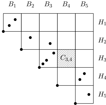
Figure 3: The grid decomposition of the permutation \pi = 131415101267811931452 . The image of \pi under the bijection of Theorem 4.9 is the restricted growth function \phi(\pi) = 111223332345445 .
