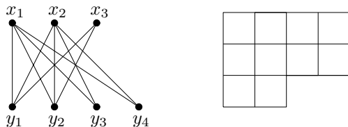
FIGURE 1. A Ferrers graph and its associated Ferrers shape \lambda = (4, 4, 2) .
