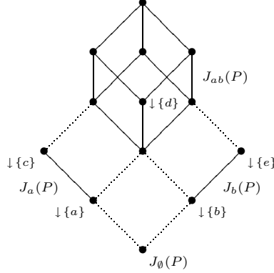
FIGURE 1. The partition of J(P) for P = \begin{smallmatrix} c \\ \setminus_a^d \\ \setminus_b^e \end{smallmatrix}
